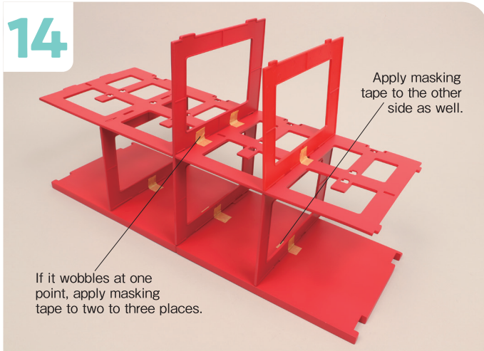
We can temporarily affix the parts with masking tape at this stage of assembly. First, apply masking tape to the seams on top where the Base Plates and Shelving meet the Partitions as shown.
