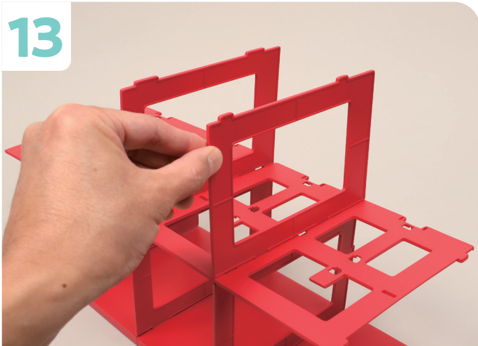
Insert its bottom protrusions into the holes in the Shelving as you did with the other Partitions.
